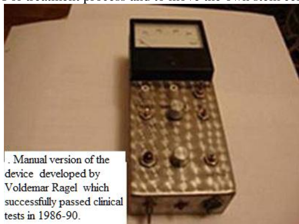
Device (manual drive version).
